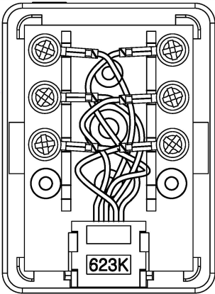
623K Jack - Surface Mount
