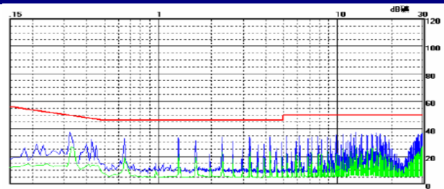
VRA2405LD-20WR2 CE (Negative line)
