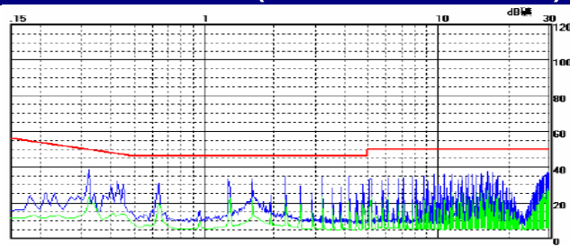
VRA2405LD-20WR2 CE (Positive line)
