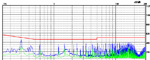
VRA4815LD-20WR2 CE (Positive line)
