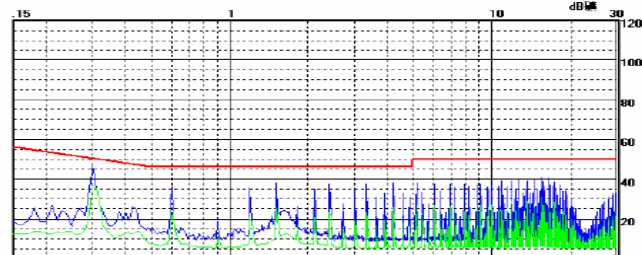
VRA4815LD-20WR2 CE (Negative line)
