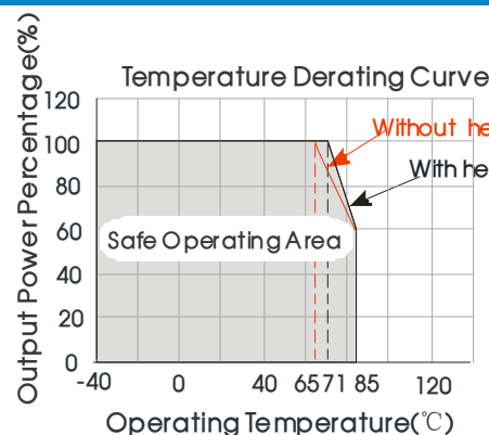
Operating Temperature, Except URB1D03/05LMD-20W(H)R3(A2S/A4S)
