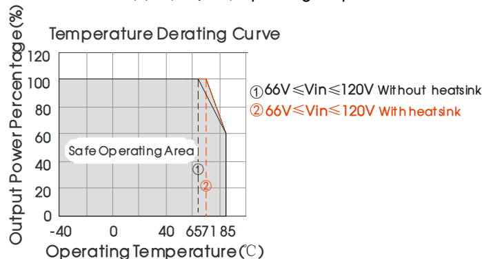
URB1D03LMD-20W(H)R3(A2S/A4S) Operating Temperature
