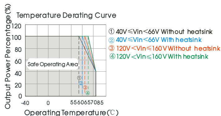
Operating Temperature, Except URB1D03/05LMD-20W(H)R3(A2S/A4S)
