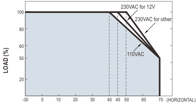
AMBIENT TEMPERATURE WITH CONDUCTION COOLING(°C)
