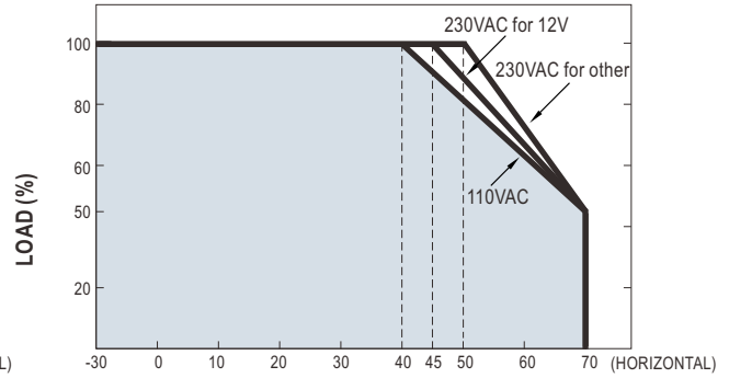
AMBIENT TEMPERATURE WITH FORCED AIR COOLING(°C)
