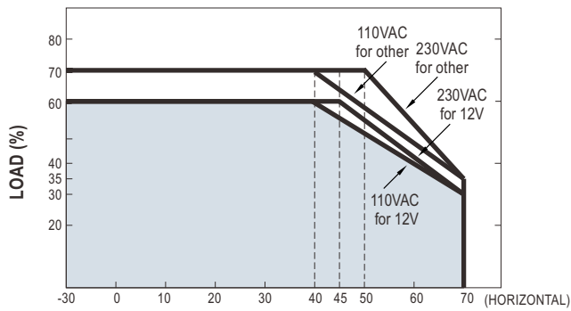
AMBIENT TEMPERATURE WITH CONVECTION COOLING(°C)
