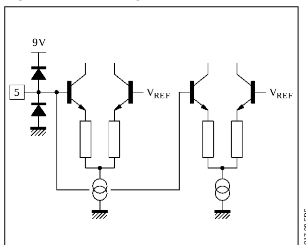
Figure 7 : Pin 5 Configuration
