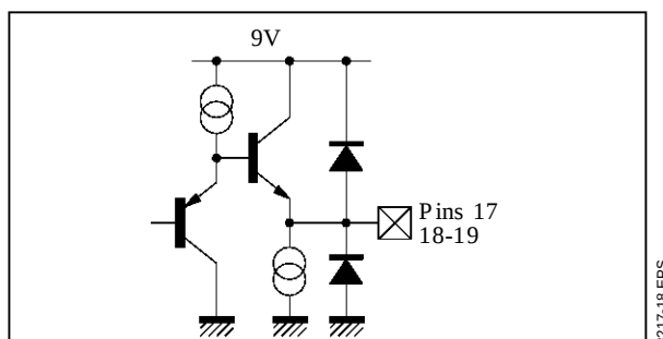
Figure 16 : Pins 17 - 18 - 19 Configuration
