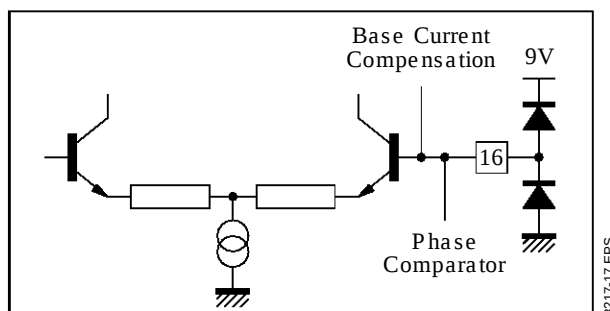
Figure 15 : Pin 16 Configuration
