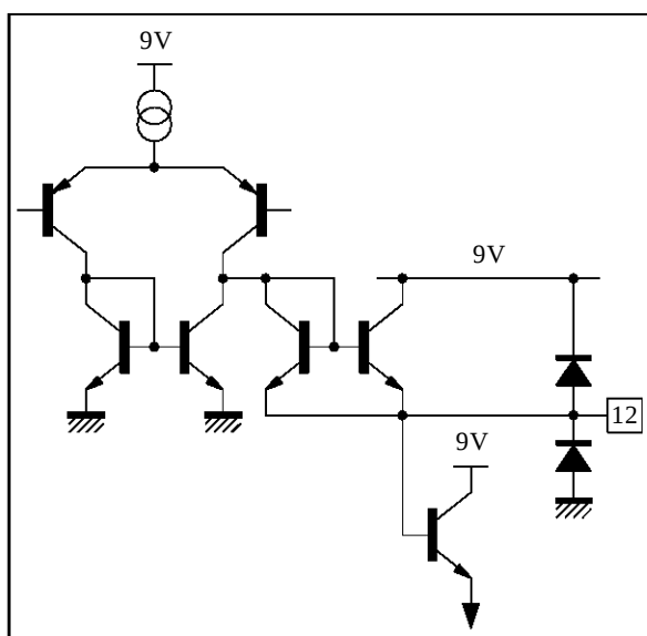
Figure 12 : Pin 12 Configuration
