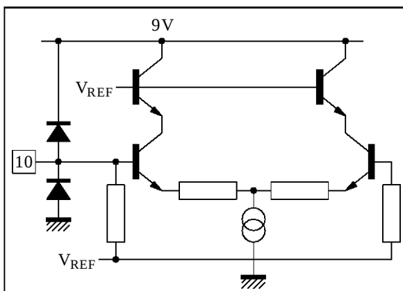
Figure 11 : Pin 10 Configuration
