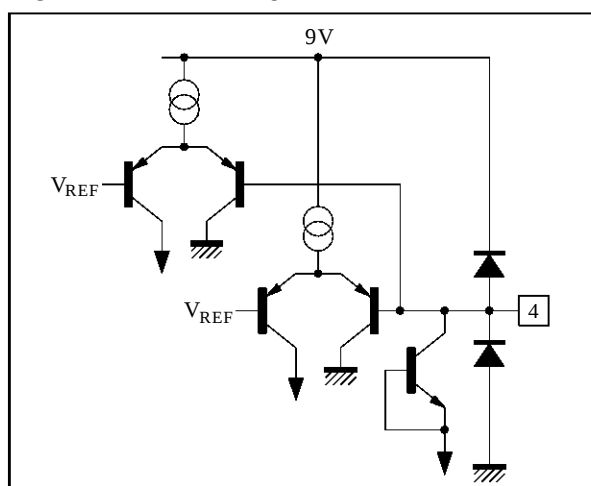
Figure 6 : Pin 4 Configuration
