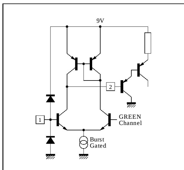
Figure 6 : Pin 4 Configuration
