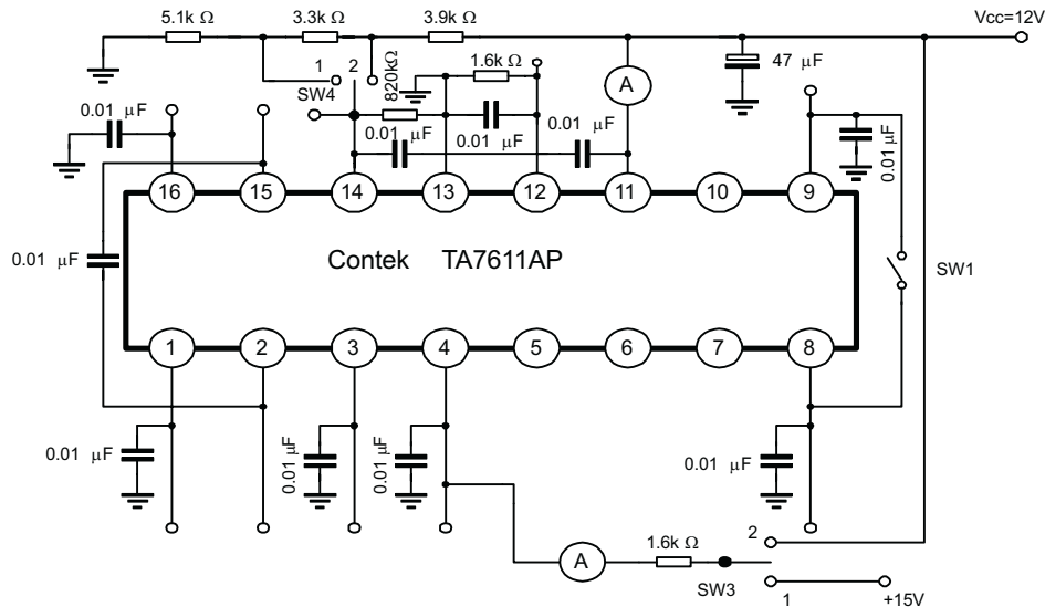
TEST CIRCUIT 2
