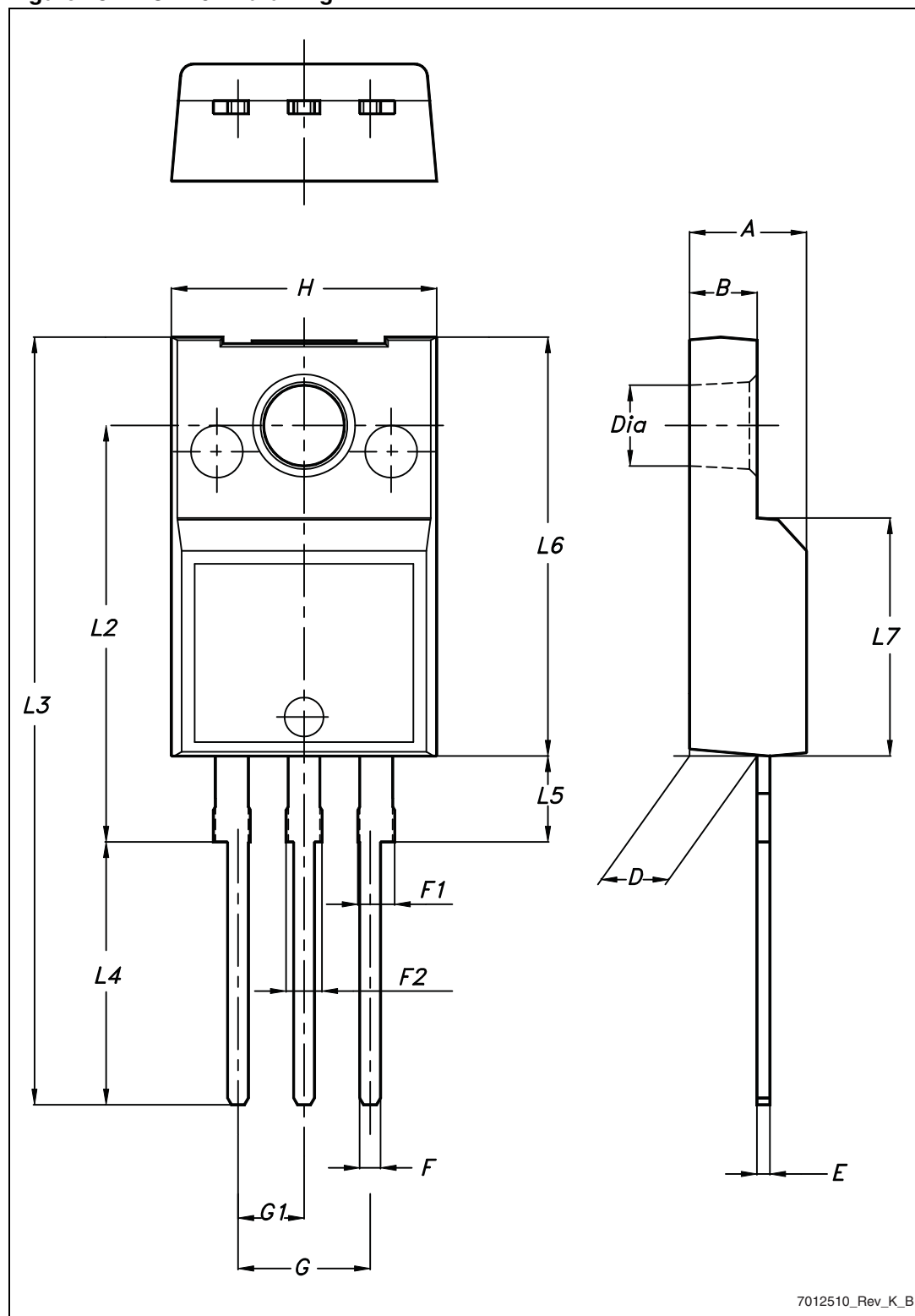
Figure 28. TO-220FP drawing
