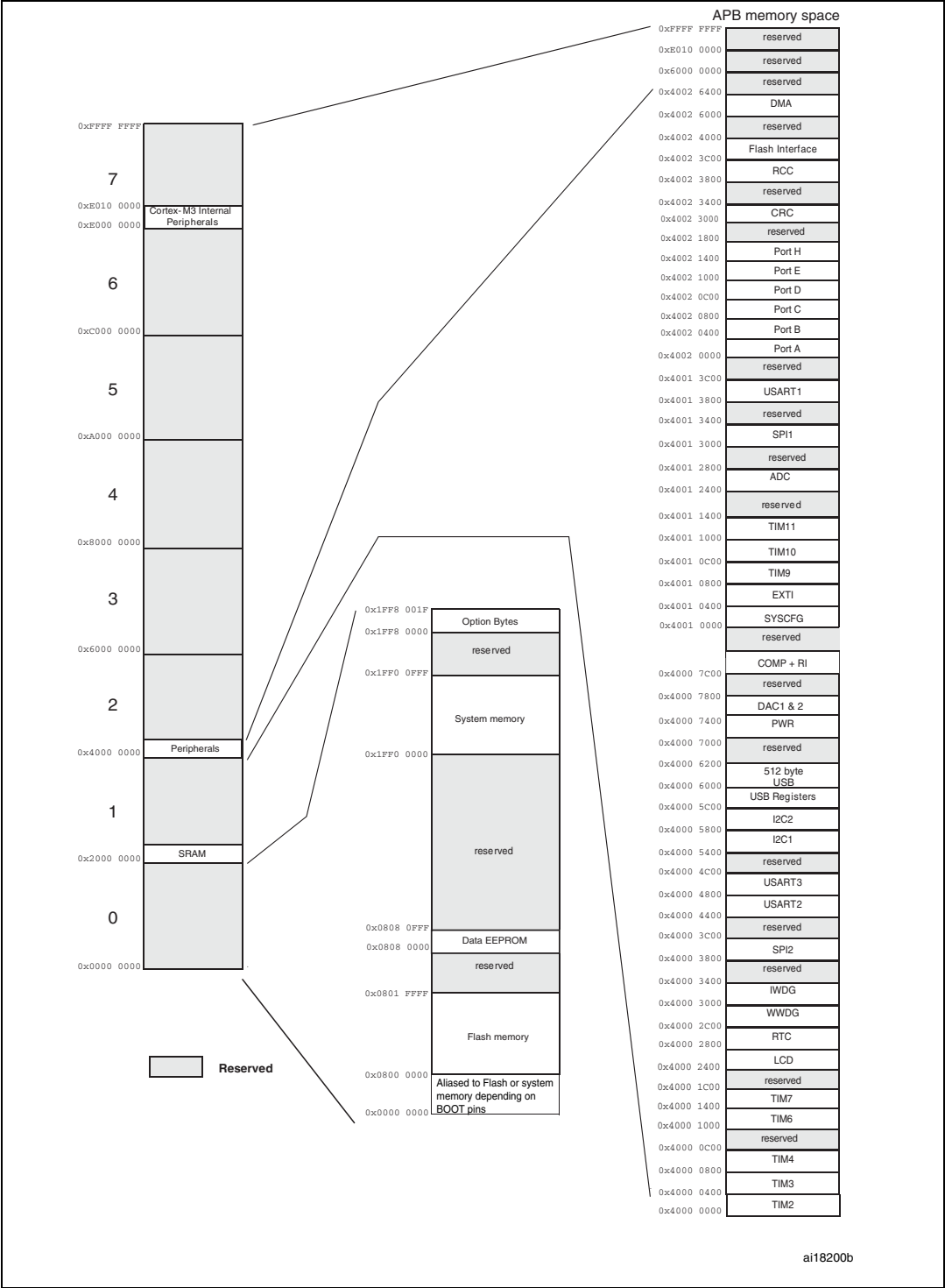
Figure 9. Memory map
