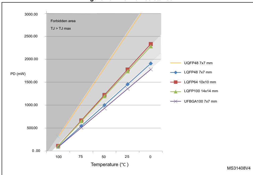
Figure 43. Thermal resistance
