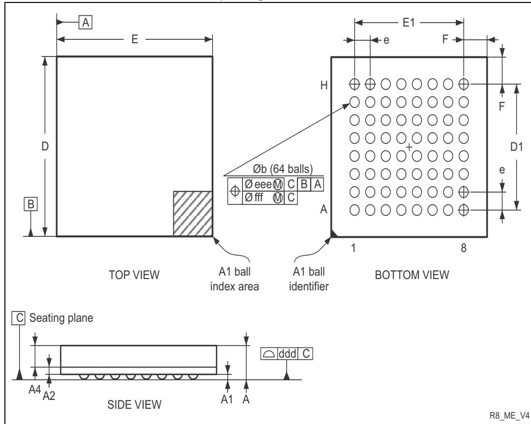
Figure 43. TFBGA64 – 64-ball, 5 x 5 mm, 0.5 mm pitch thin profile fine pitch ball array package outline
