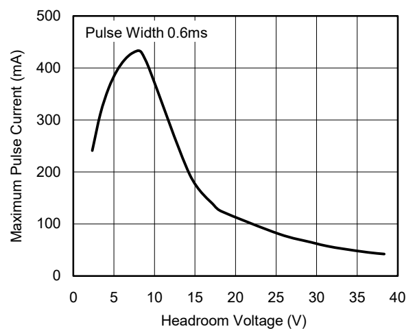
Maximum Pulse Current vs. Headroom Voltage
