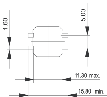
PCB footprint, view on component side
