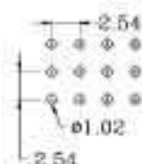
Recommended P.C.Board Hole Layout
