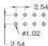
Recommended P.C.Board Hole Layout
