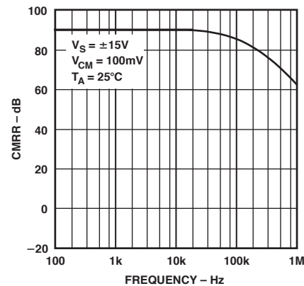
TPC 18. OP282 Common-Mode Rejection Ratio (CMRR) vs. Frequency
