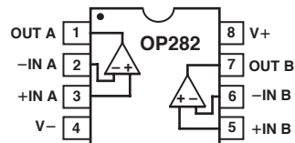
8-Lead Epoxy DIP (P Suffix)
