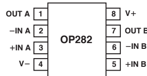
8-Lead Narrow-Body SOIC (S Suffix)
