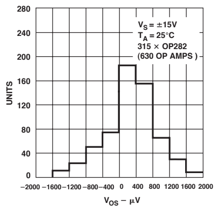
TPC 19. V_{OS} Distribution "P" Package
