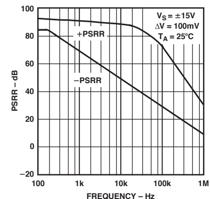
TPC 15. OP282 Power Supply Rejection Ratio (PSRR) vs. Frequency
