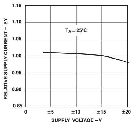
TPC 10. Relative Supply Current vs. Supply Voltage
