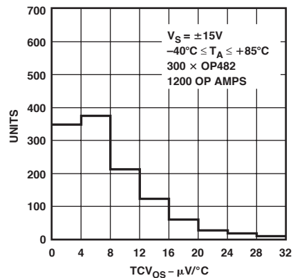
TPC 21. TCV_{OS} Distribution "P" Package
