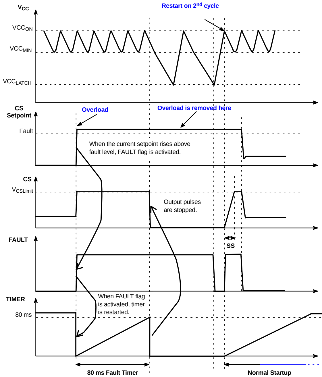
Figure 4. Overload
