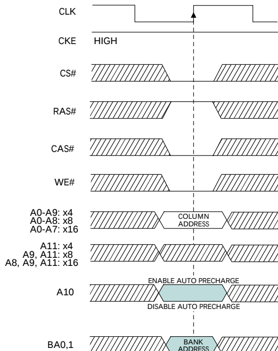
Figure 13 WRITE Command
