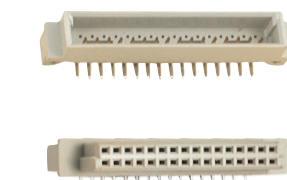
32 PIN SIZE DIP RIGHT ANGLE (DUAL ROWS)
