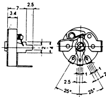
P6890 20mm VARIABLE RESISTOR 150VAC 0.1W
