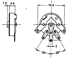
P6880 20mm VARIABLE RESISTOR 100VAC 0.05W
