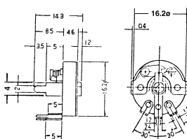
P6893 60mm VARIABLE RESISTOR 500VAC 0.5W
