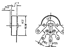
P6891 20mm VARIABLE RESISTOR 150VAC 0.1W
