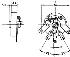
P6881 20mm VARIABLE RESISTOR 100VAC 0.05W
