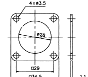
M595729C RUBBER PLATE FOR M30 CIRCULAR CONNECTOR (FOR M595723 M595727)
