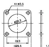
M595719C RUBBER PLATE FOR M22 CIRCULAR CONNECTOR (FOR M595713 M595717)
