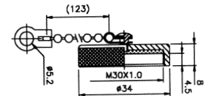
M595728 PROTECTIVE CAP FOR M30 CIRCULAR CONNECTOR (FOR M595723 M595727)
