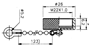
M595718 PROTECTIVE CAP FOR CIRCULAR M22 CONNECTOR (FOR M595713 M595717)
