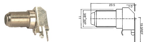
M564255 RIGHT ANGLE F FEMALE PCB MOUNT
