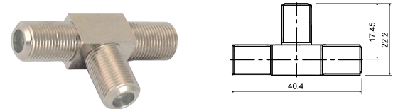
M56422 F FEMALE (RG59U/5C2V)
