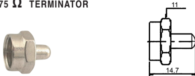
M5631 F MALE DUMMY LOAD 75 \Omega TERMINATOR
