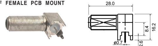
M56426 RIGHT ANGLE F FEMALE PCB MOUNT
