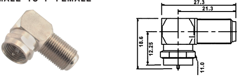
M5640 RIGHT ANGLE F FEMALE TO F MALE QUICK TYPE
