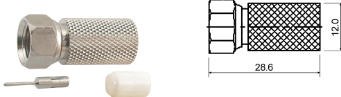
M5629 F QUICK CONNECTOR TWIST ON TYPE (RG58U/59U)
