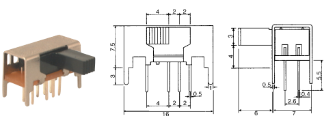
B15830 SLIDE SWITCH (6P3T)
