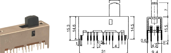
B15830 SLIDE SWITCH (6P3T)
