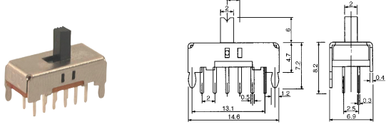
B15800 SLIDE SWITCH (4P2T)
