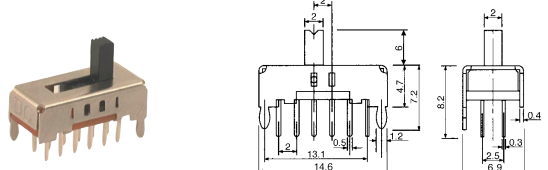
B15780 SLIDE SWITCH (2P4T)
