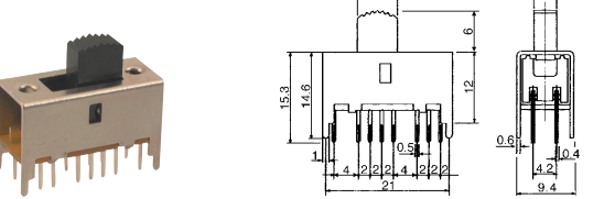
B15810 SLIDE SWITCH (4P3T)
