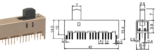
B15840 SLIDE SWITCH (8P3T)
