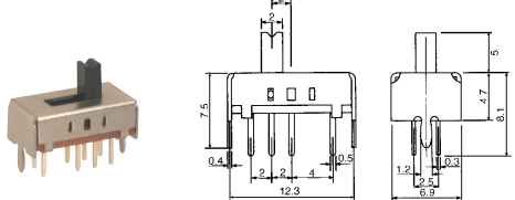
B15810 SLIDE SWITCH (4P3T)
