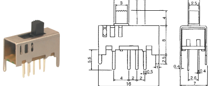
B15840 SLIDE SWITCH (8P3T)
