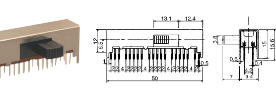
B15850 SLIDE SWITCH (8P4T)
