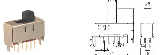
B1576 SLIDE SWITCH (2P3T)
