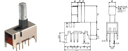
B15850 SLIDE SWITCH (8P4T)
