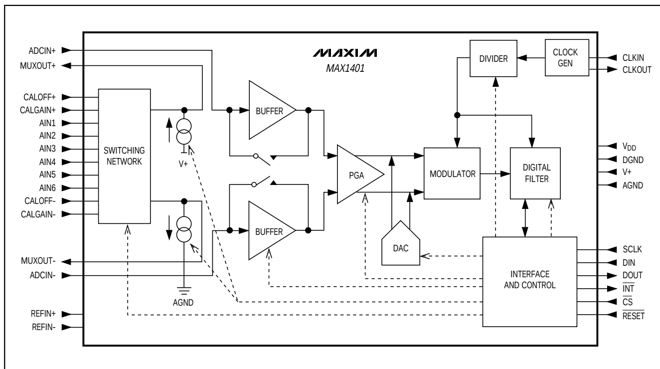
Figure 2. Functional Diagram
