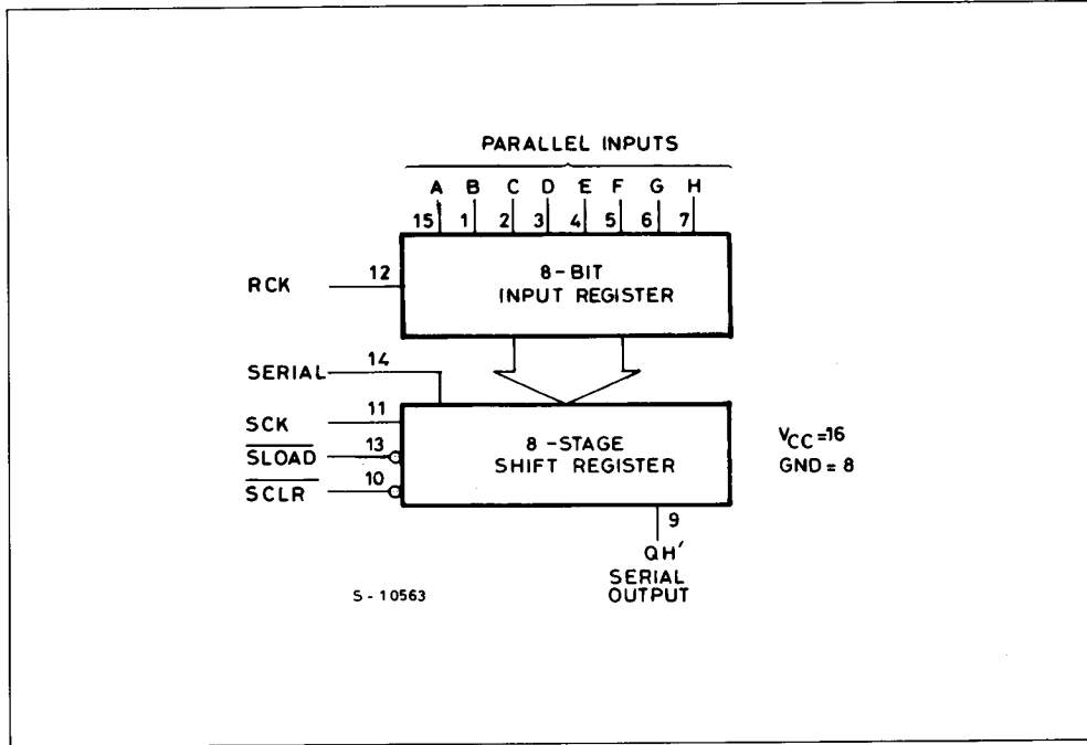
BLOCK DIAGRAM
