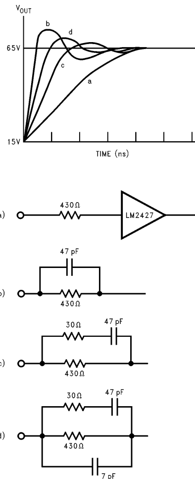
FIGURE 2. Influence of Input Networks on Switching Performance
