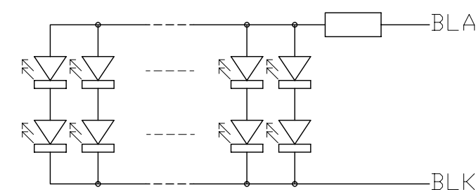
Backlight Circuit (No. of LEDs = 2x18pcs) Scale=free
