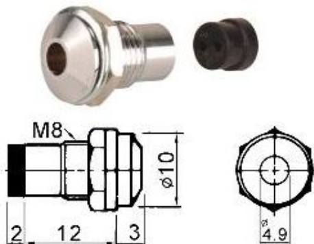
R7878962 5mm LED HOLDER
