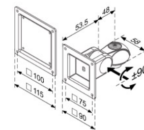
LA-511 Universal Joint
