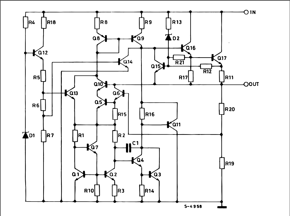
Figure 3. Schematic diagram
