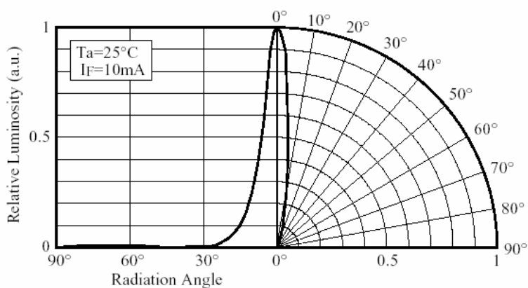
■ Directivity
