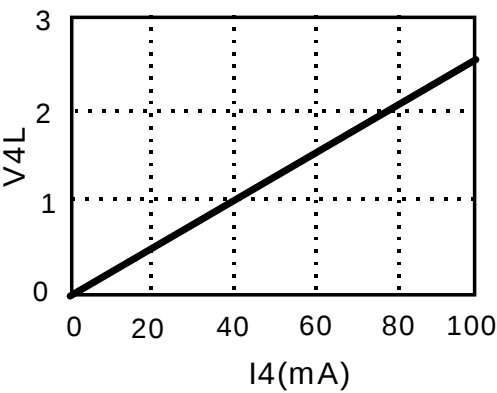
Figure 2. I4-V4L
