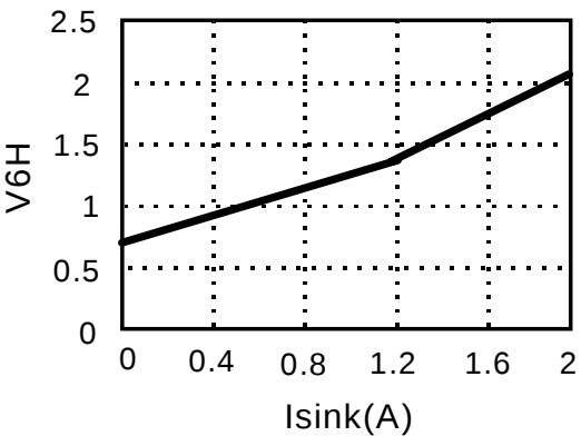
Figure 3. Isink-V6H
