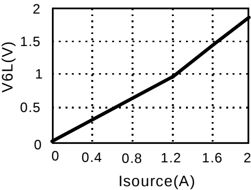
Figure 4. Isource-V6L
