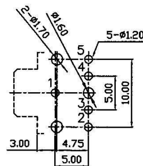
Pin Hole Layout (Jack Bottom View)
