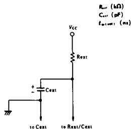
Fig.2 Timing Component Connections
