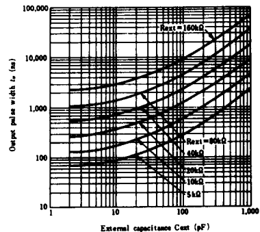
Fig.3 Typical Output Pulse Width ( C_{ext} \leq 1000\text{pF} )
