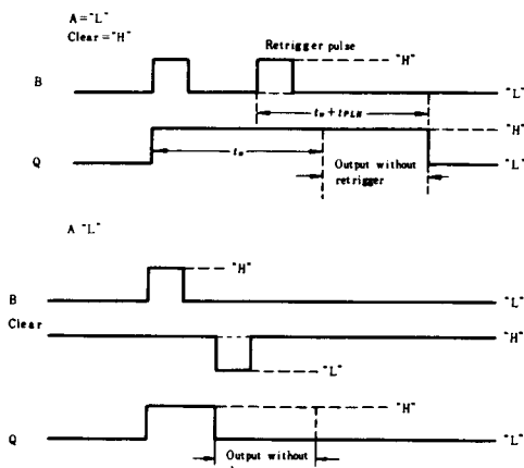
Fig.1 Typical Input/Output Pulses
