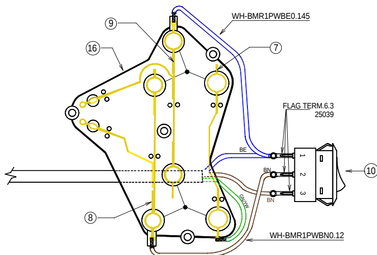
ASSEMBLY EXTENSION REEL TERMINAL HOUSING
