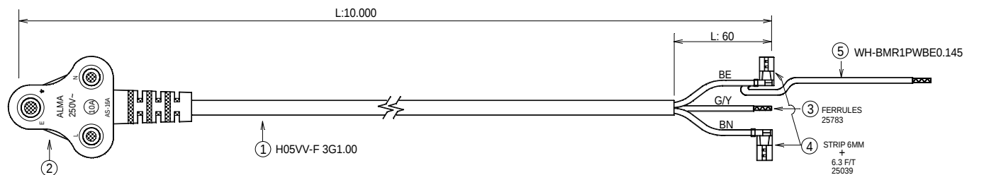
ASSEMBLY EXTENSION REEL TERMINAL HOUSING
