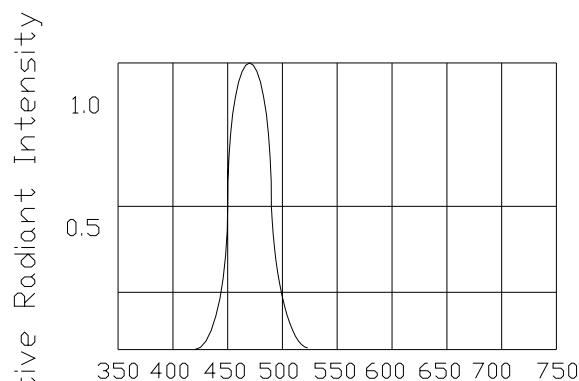
Wavelength (nm) Spectral Distribution BLUE
