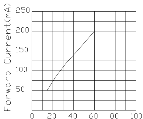
Junction Temperature (°C) BLUE
