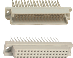
48 Pin size wire wrap (triple rows)
