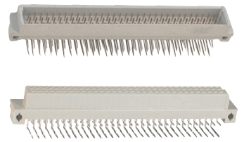
64 Pin size DIP right angle (dual rows)
