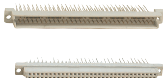
64 Pin size wire wrap (dual rows)
