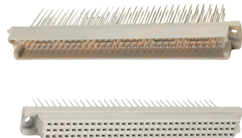
96 Pin size wire wrap (triple rows)
