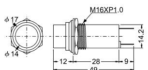
R735R /G /Y 5mm LED indicator light 2V W/O resistor R:red G:green Y:yellow
