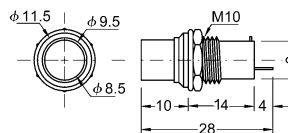
R733R /G /Y 5mm LED indicator light 2V W/O resistor R:red G:green Y:yellow
