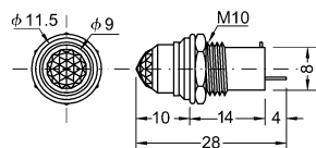
R732R /G /Y 3mm LED indicator light 2V W/O resistor R:red G:green Y:yellow
