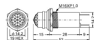
R736R /G /Y 5mm LED indicator light 2V W/O resistor R:red G:green Y:yellow
