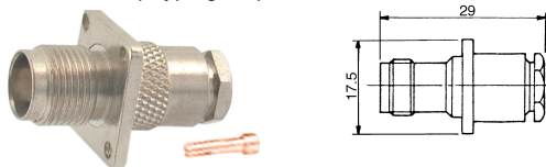
M57705 TNC female to TNC male push on gold-pin
