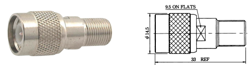
M57719 TNC male to F female gold-pin
