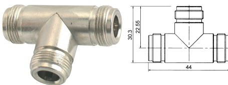
M5728 T-type triple N female gold-pin
