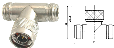
M5727 T-type N male to double N female gold-pin
