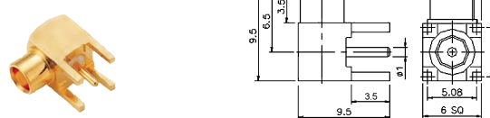
M52250 MCX female surface mount (gold plated)
