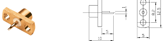
M52192 MCX female chassis mount (gold plated)
