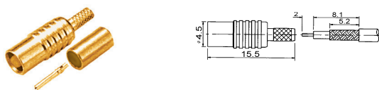
M52166 MCX female bulkhead crimp type (RG174U/178U) (gold plated)
