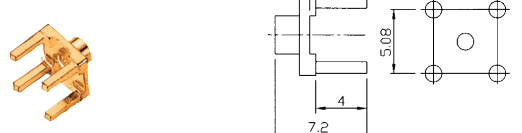
M52220 MCX PCB terminal (RG402U/405U) (gold plated)
