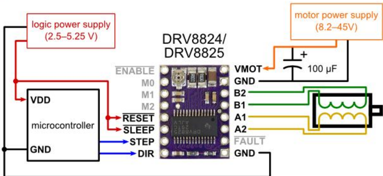
Schematic diagram for the DRV8824/DRV8825 stepper motor driver carrier.
