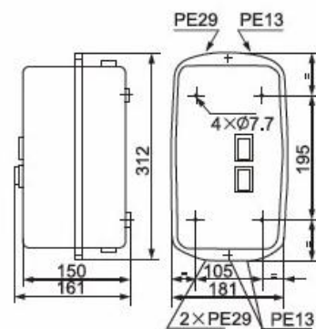
LE-D40~LE-D95
