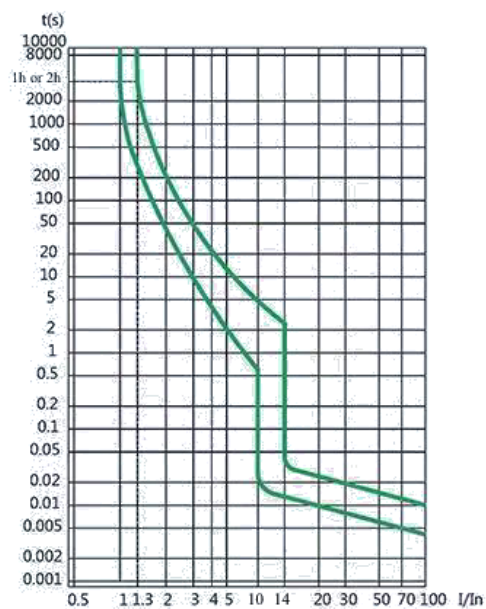
D Curve
