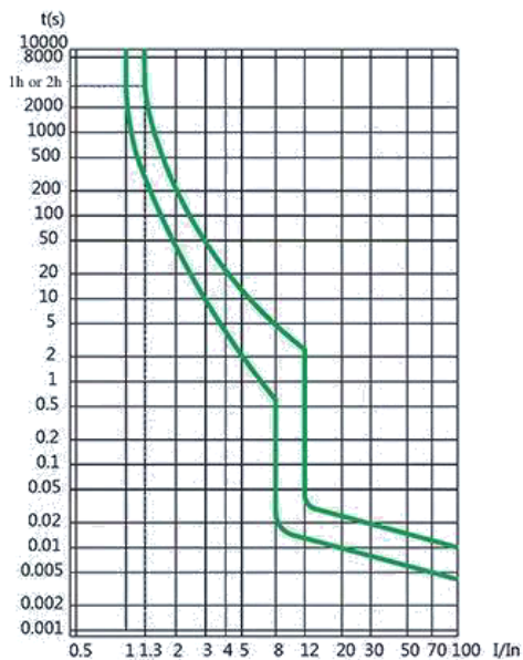
C Curve
