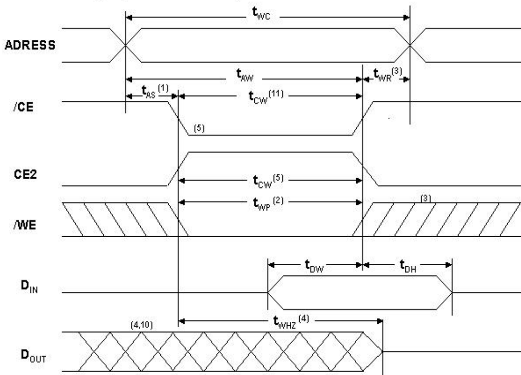
WRITE CYCLE 2 (Chip Enable Controlled)
