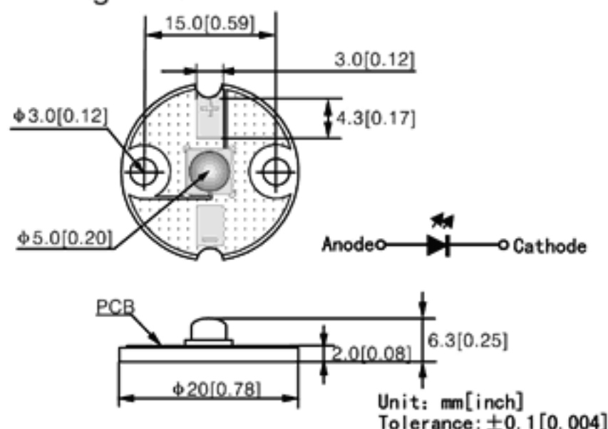
Package Dimension:
