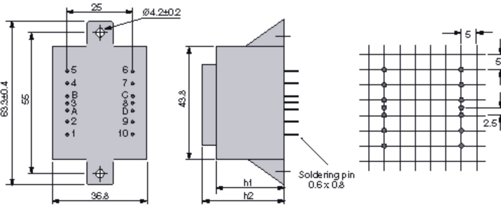
Dimensions of drawing without tolerances ± 0,3 mm. soldering pins 0,6 x 0,8 mm
