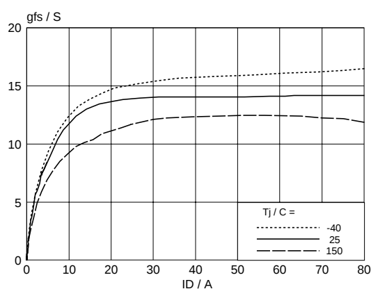
Fig.8. Typical transconductance, T_j = 25\text{ °C} . g_{fs} = f(I_D) ; conditions: V_{DS} = 15\text{ V}
