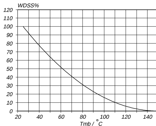
Fig.15. Normalised avalanche energy rating. W_{DSS}\% = f(T_{mb}) ; conditions: I_D = 41 A
