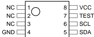
8-lead TSSOP
