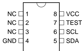
8-lead PDIP
