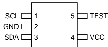
5-lead SOT23
