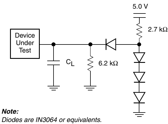
Figure 8. Test Setup
