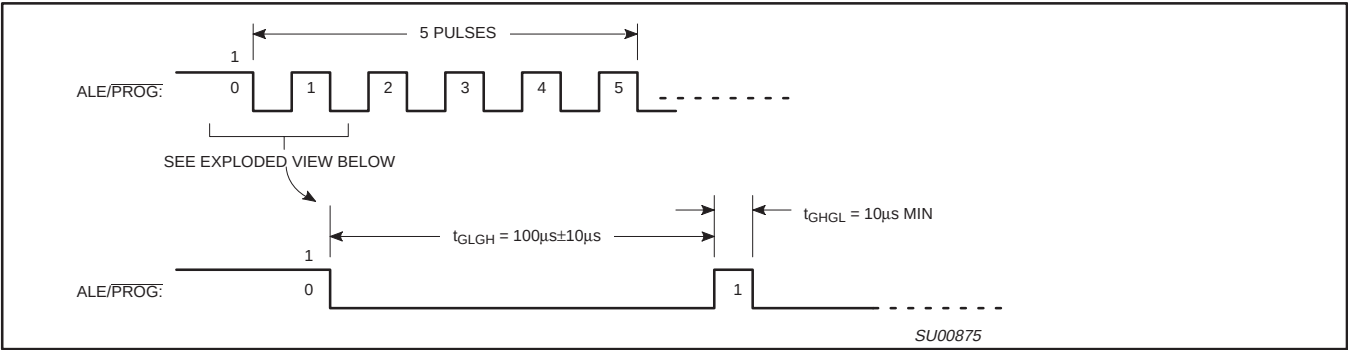
Figure 27. PROG Waveform
