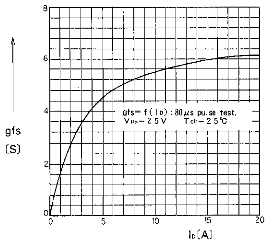
Typical Forward Transconductance vs. I_D
