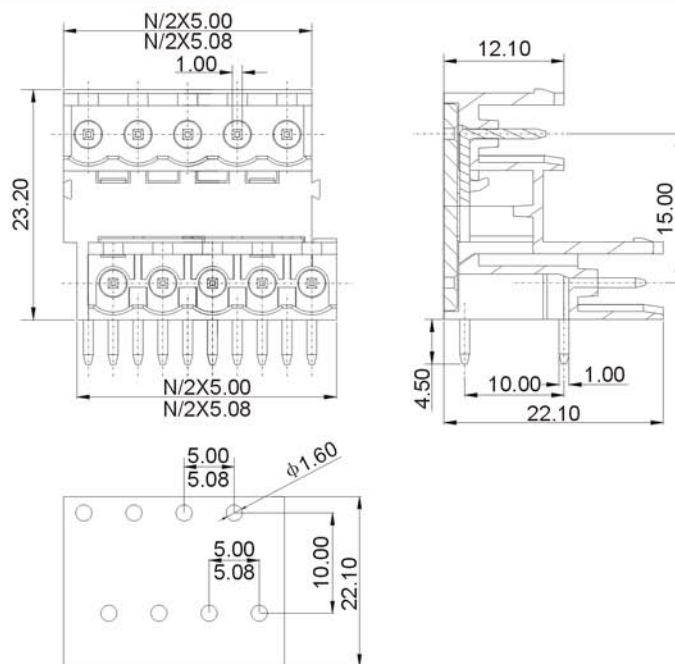
PCB LAYOUT
